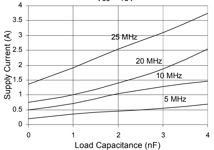
Fig. 13 Supply Current vs. Load Capacitance V cc = 15V
