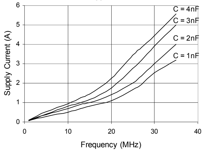
Fig. 11 Supply Current vs. Load Capacitance V cc = 8V
