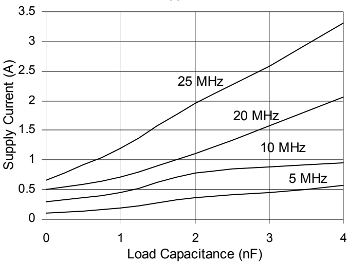
Fig. 12 Supply Current vs. Load Capacitance V cc = 12V
